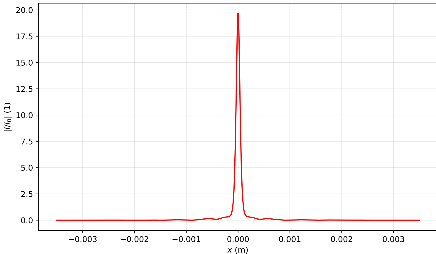
Intensity profile I(x, y = 0, z = 0.478)/I_0 , P_{in}=2.0P_{cr} , artificial time
